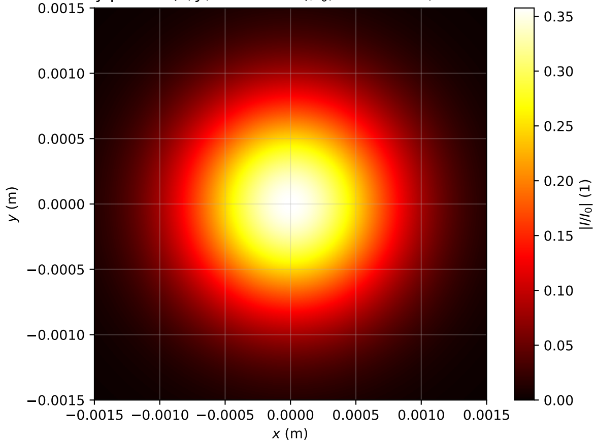
Intensity profile I(x, y, z = 2.866m)/I_0 , P_{in}=0.1P_{cr} , artificial time
